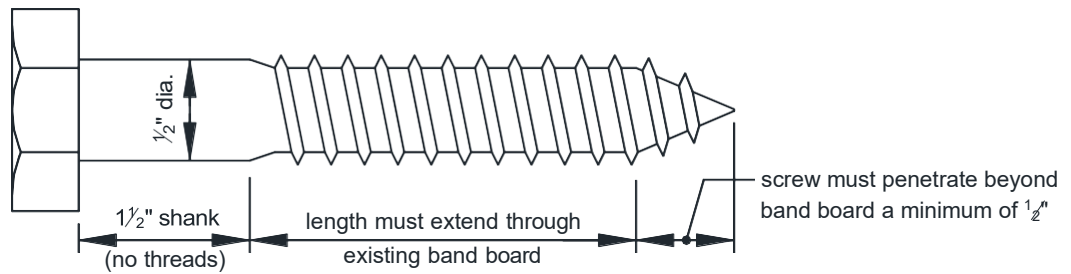
FIGURE 27: LAG SCREW
