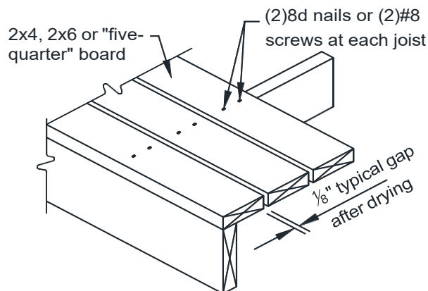
FIGURE 1: TYPICAL DECKING
