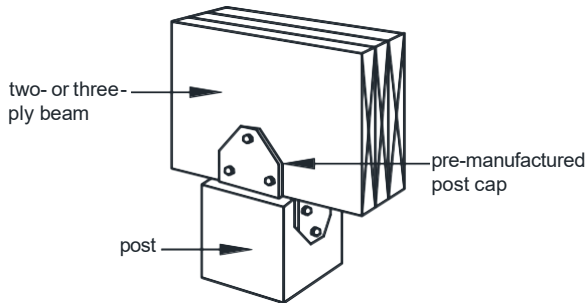
FIGURE 19: POST CAP CONNECTION
