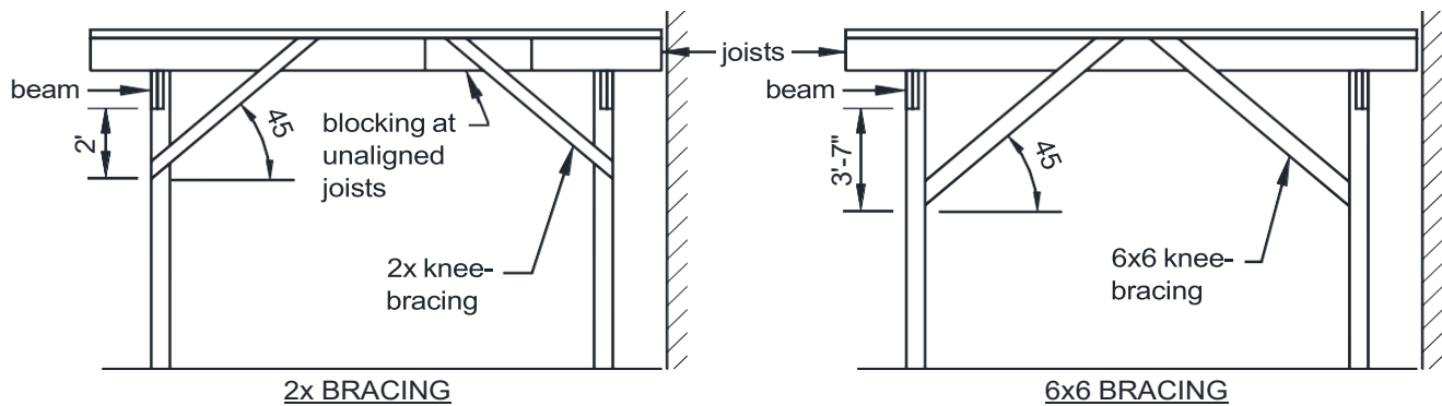
FIGURE 31: METHOD 3-KNEE-BRACING AT JOIST-POST LOCATIONS BRACING-TO-FRAMING CONNECTIONS
