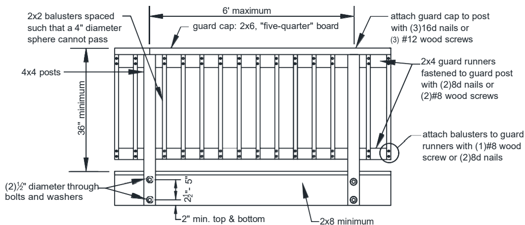
FIGURE 35: GUARD CONSTRUCTION
