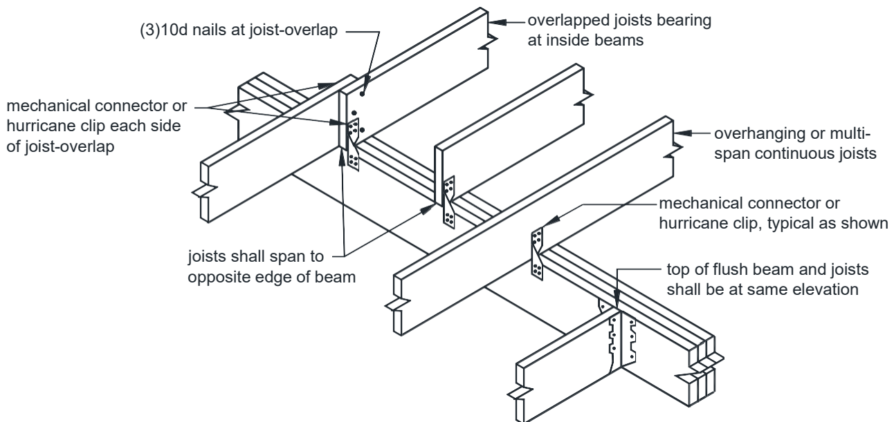
FIGURE 12: JOIST-TO-BEAM CONNECTION
