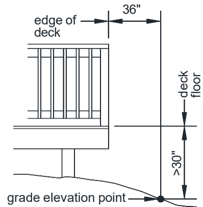
FIGURE 34: WHEN A GUARD IS REQUIRED
