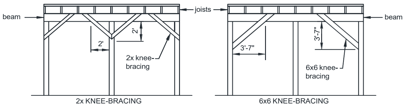
FIGURE 30: METHOD 2 - KNEE-BRACING AT BEAM-POST LOCATIONS
