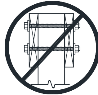
FIGURE 20: PROHIBITED CONNECTION
