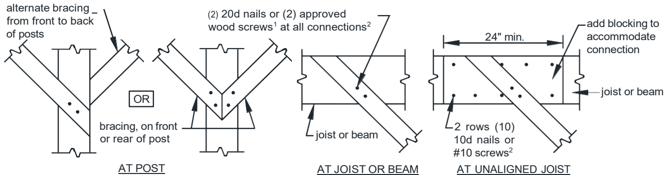
FIGURE 31: METHOD 3-KNEE-BRACING AT JOIST-POST LOCATIONS BRACING-TO-FRAMING CONNECTIONS
