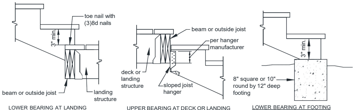
FIGURE 40: STRINGER BEARING
