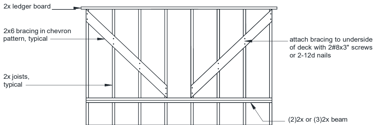
FIGURE 3: HORIZONTAL BRACING IN A CHEVRON PATTERN
