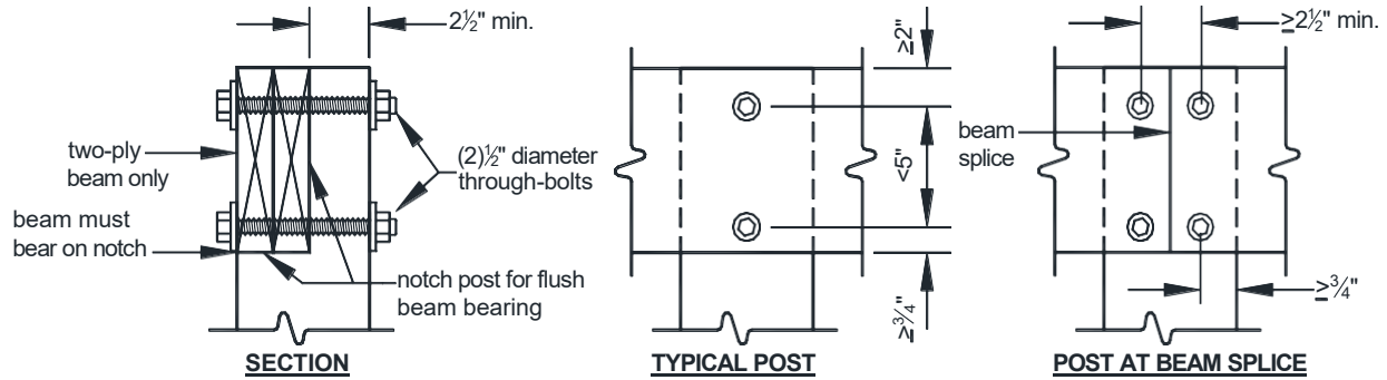
FIGURE 18: NOTCHED 6x6 POST-TO-BEAM CONNECTION
