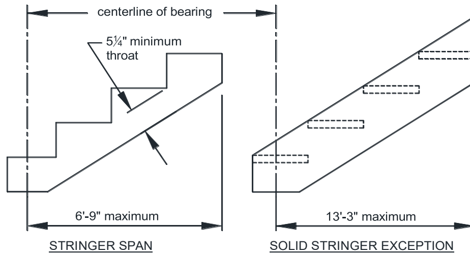
FIGURE 41: MAXIMUM STRINGER SPAN LENGTH
