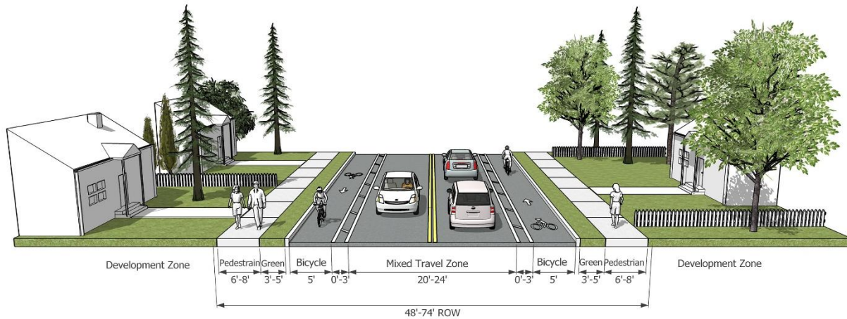
Figure 7. Collector Street with Separate Pedestrian and Bicycle Facilities
