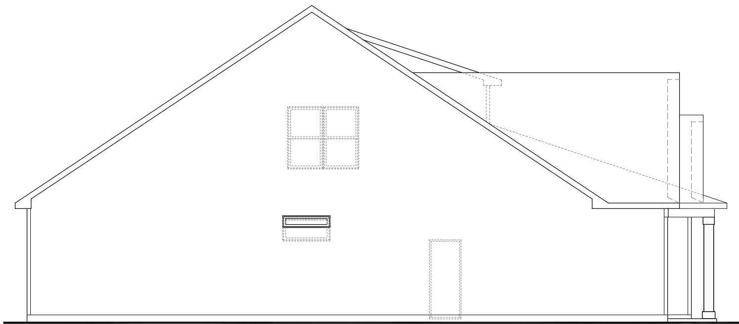
LEFT ELEVATION
