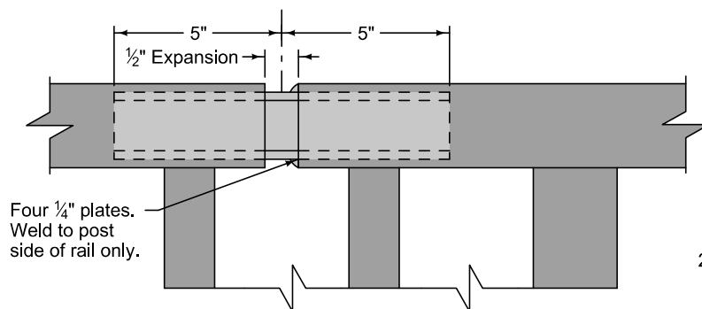
EXPANSION SLEEVE DETAIL ①
