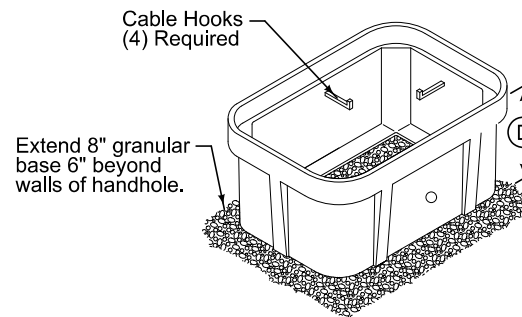
PRECAST CONCRETE COMPOSITE HANDHOLE
