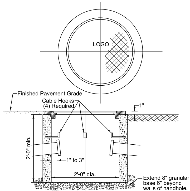
PRECAST CONCRETE HANDHOLE (TYPE I)
