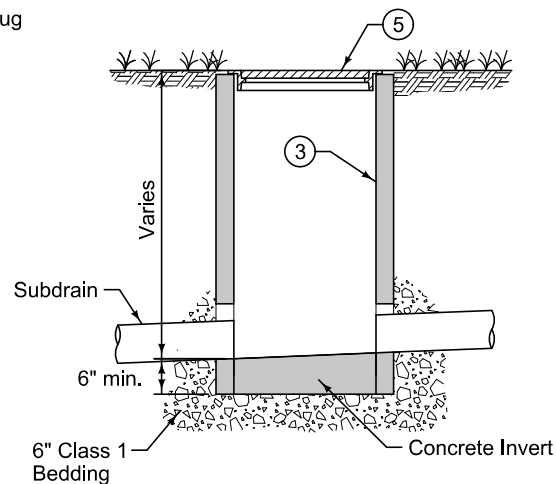
TYPE B CLEANOUT (Non-traffic areas only)
