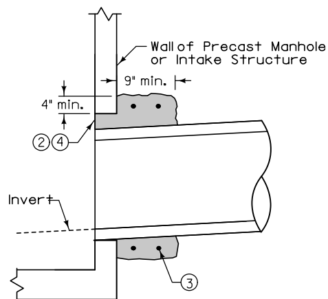
CONCRETE COLLAR FOR PIPES GREATER THAN 12"
