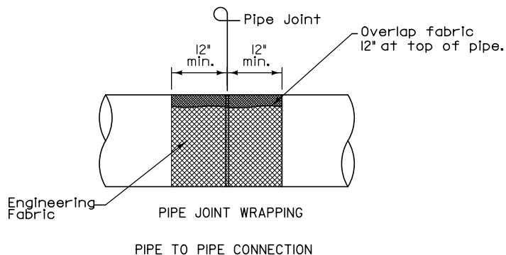
PIPE TO PIPE CONNECTION
