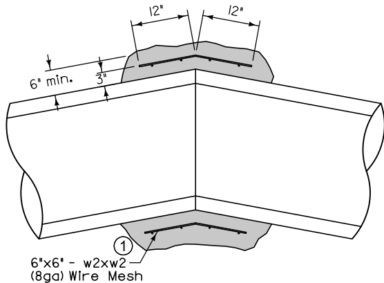
TYPE PC-2 CONCRETE COLLAR CONNECTION
