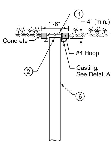
TYPE A-1 CLEANOUT
