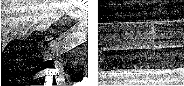
Figure 10. When researchers pulled back the porch ceiling, they found the wall board was missing so nothing was covering the insulation on this exterior wall. An air barrier of rigid foam board was put in place with spray foam (Image: Moriarta 2008).
