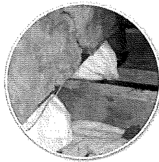
Figure 6. Air seal floor joist cavities under kneewalls by filling cavities with fiberglass batts that are rolled and stuffed in plastic bags (as shown here) or use rigid foam, Oriented Strand Board (OSB), or other air barrier board cut to fit and sealed at the edges with caulk.
