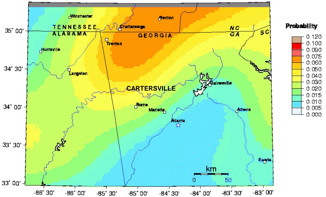
GMT May 3 21 09 Earthquake probabilities from USGS 2002 PSHA. 50 km maximum horizontal distance. Site of interest: triangle. Epicenters m > 5 black circles; rivers blue.
